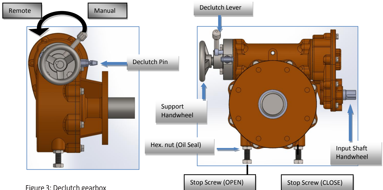
Figure 3: Declutch gearbox
