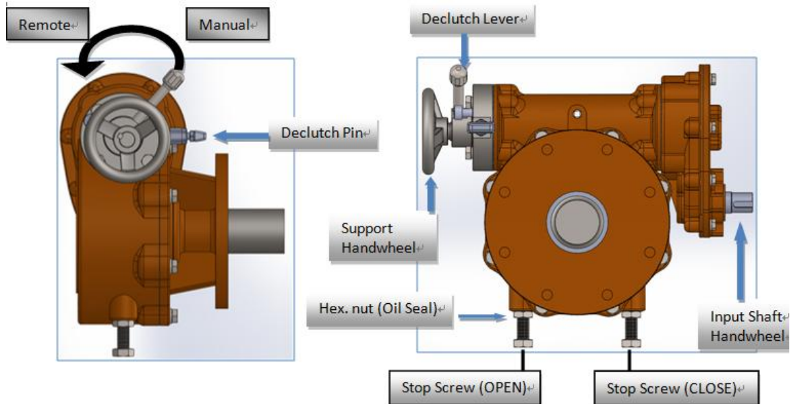
Figure 4: Declutch gearbox
